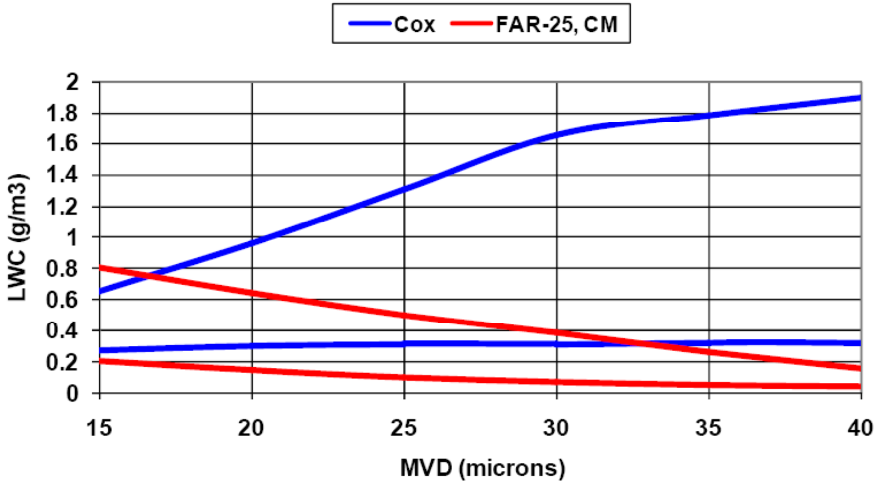
Cox & Co., Inc., Icing Envelope versus FAR-25 Continuous Maximum (CM) Test Section-1 @ 200 mph NASA "Mod-1" nozzles, Single nozzle pattern, November 2011 Calibration
