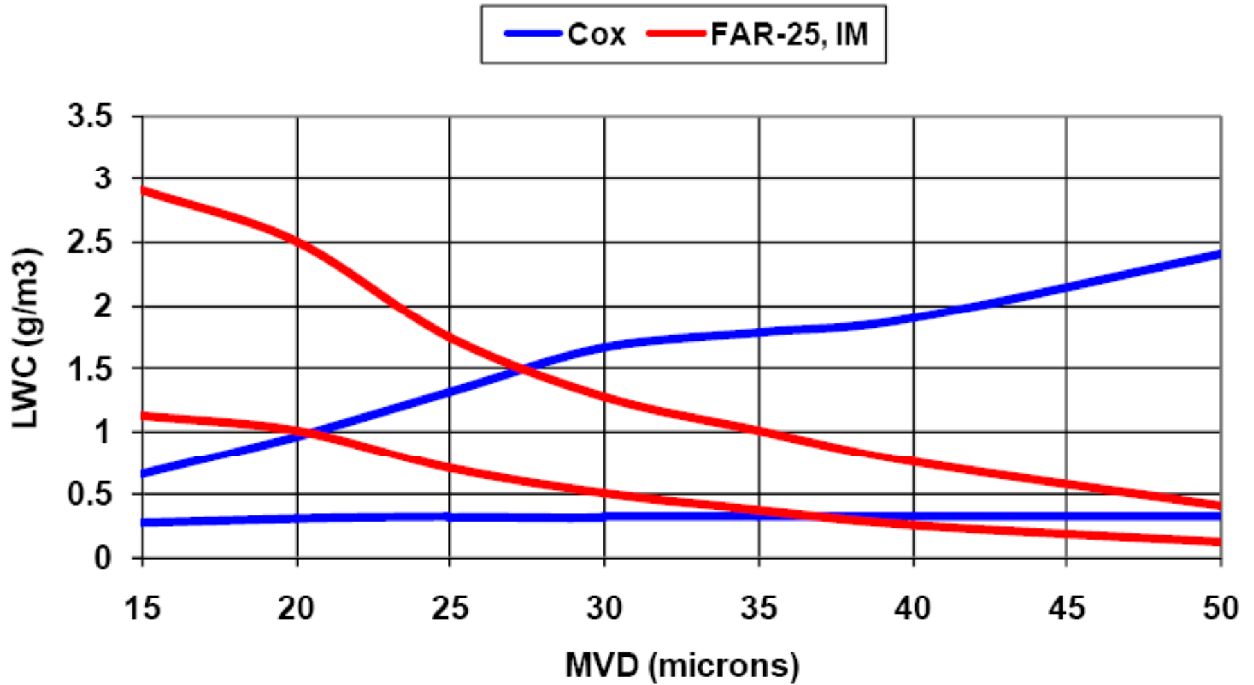
Cox & Co., Inc., Icing Envelope versus FAR-25 Intermittent Maximum (CM) Test Section-1 @ 200 mph NASA "Mod-1" nozzles, Single nozzle pattern, November 2011 Calibration
